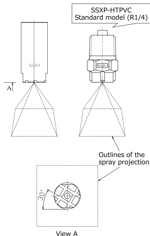
Fig. 1 Square spray pattern orientation
